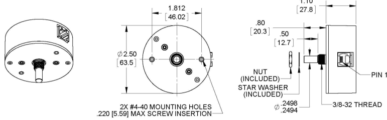
A2 Absolute Optical Shaft Encoder Bushing Version
