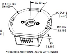
R-OPTION BASE (ROTATIONAL MOUNTING)
