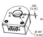
A-OPTION BASE (ALIGNMENT BOSS)
