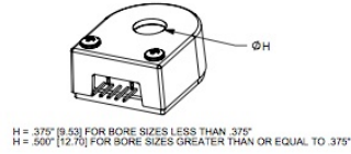
G-OPTION BASE (1.812" MOUNTING)
