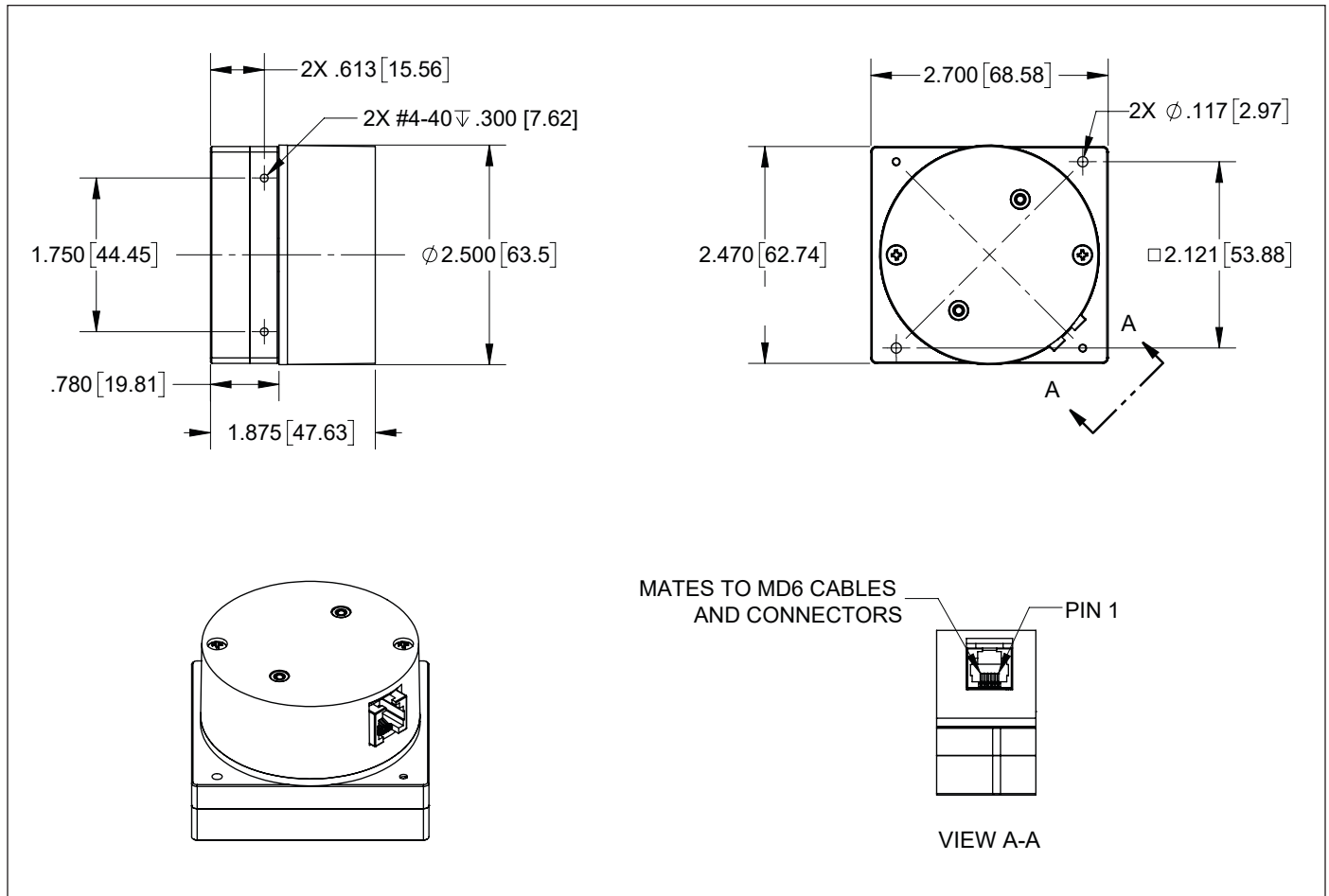
A2T Absolute Optical Inclinometer
