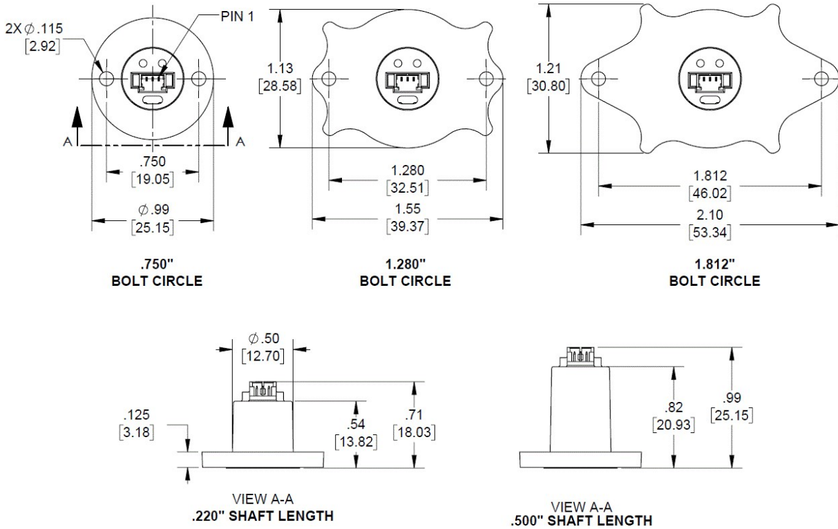
MAE3 Absolute Magnetic Kit Encoder
