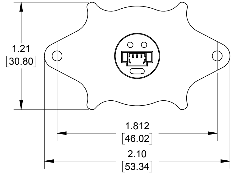
1.812" BOLT CIRCLE
