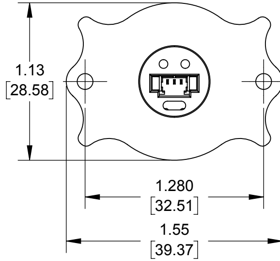
1.280" BOLT CIRCLE
