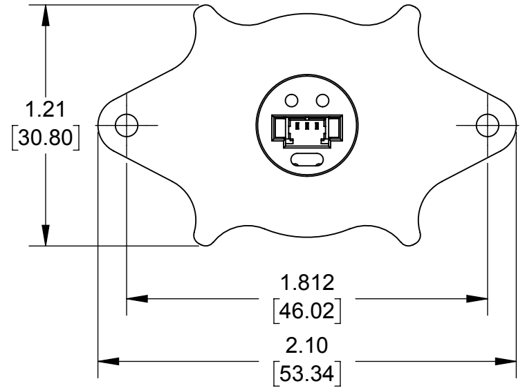
1.812" BOLT CIRCLE
