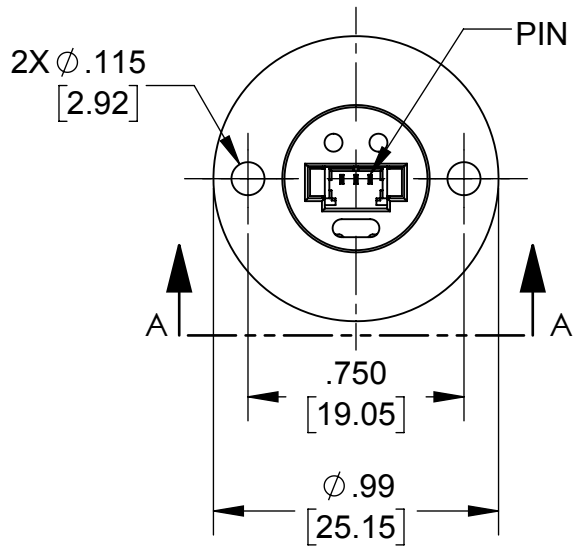
.750" BOLT CIRCLE
