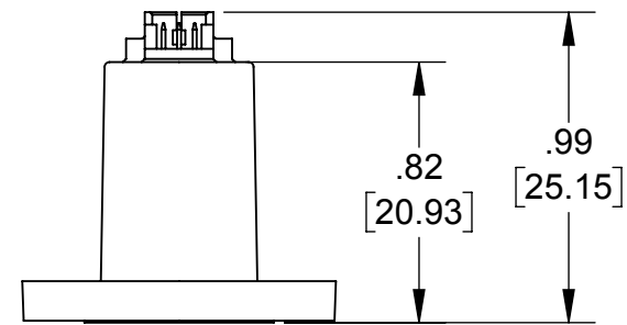
VIEW A-A .500" SHAFT LENGTH
