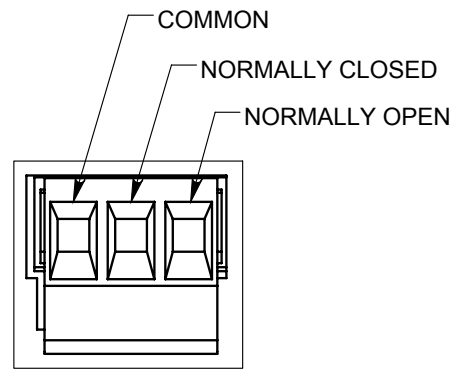
DETAIL B RELAY OUTPUT
