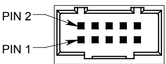
DETAIL A ENCODER INPUT DIFFERENTIAL
