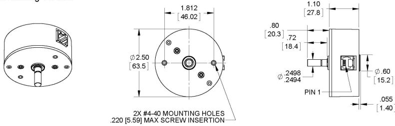
A2 Absolute Optical Shaft Encoder Ball Bearing Version
