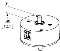
E-OPTION COVER (REAR SHAFT EXTENSION)
