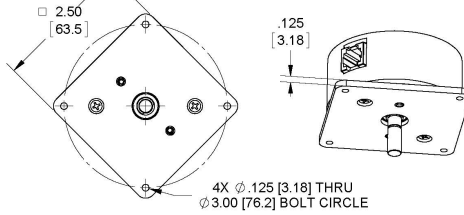
M-OPTION BASE (MOUNTING PLATE)
