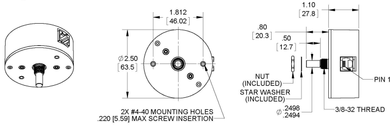
A2 Absolute Optical Shaft Encoder Bushing Version
